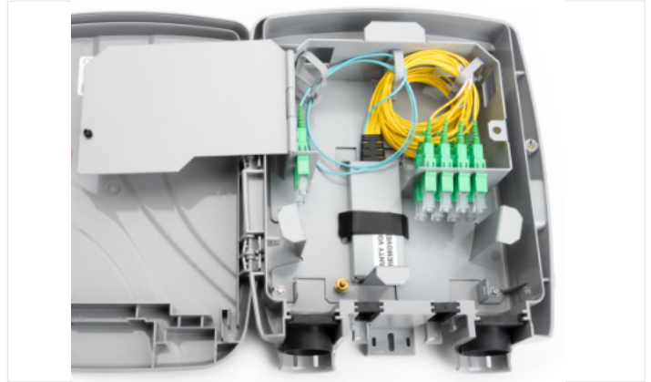
LPT Terminal with SC APC Adapter Feeder Input
