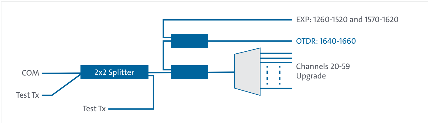
Optical Layout
